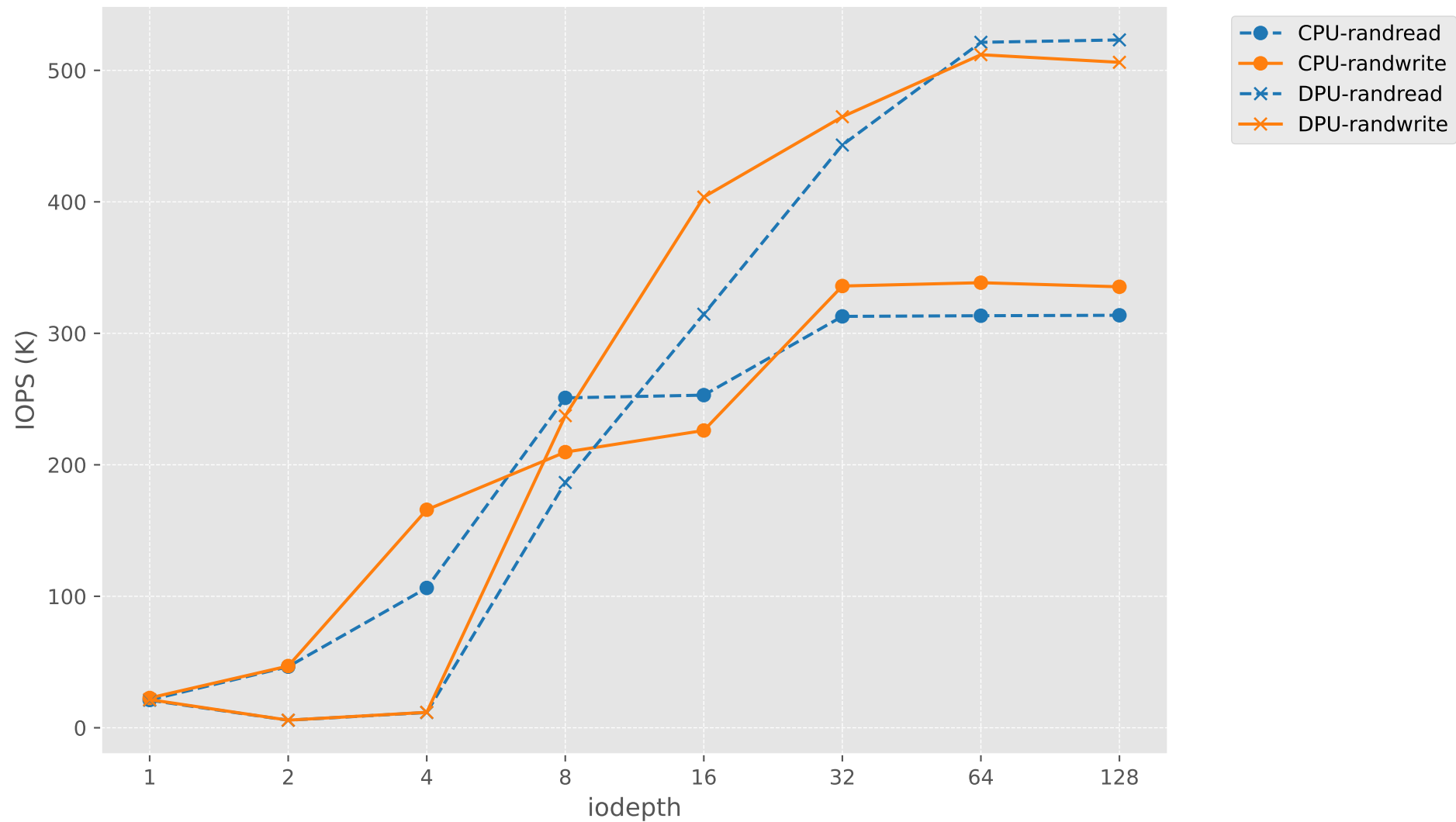
IOPS vs iodepth (Random)
